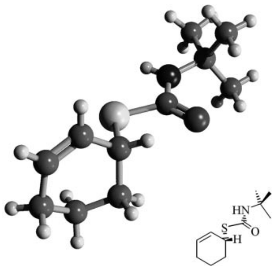
Figure 1. X-ray crystal structure of thiocarbamate (+)-( R )- 14c
