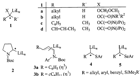
Scheme 1. Some chiral organolithium compounds 1 – 5
