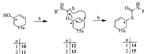
Scheme 4. Synthesis of S -allyl N -monoalkylmonothiocarbamates; reagents and conditions: (a) i) NaH, THF, 0 °C; ii) R–NCS, THF, 0 °C; iii) \text{H}_3\text{O}^+ ; (b) neat, 105–150 °C
