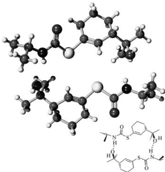
Figure 4. X-ray crystal structure of thiocarbamate rac - 21g
