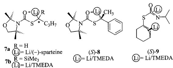
Scheme 3. Lithiated monothiocarbamates
