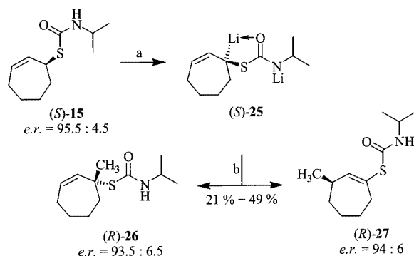
Scheme 8. Methylation of thiocarbamate (-)-(S)- 15 ; ligands at the lithium centers are omitted for the sake of clarity; reagents and conditions: (a) s BuLi/TMEDA, -78 °C, 30 min; (b) i) MeI, -78 °C, 15 h; ii) HOAc, -78 °C, 15 min; iii) NaHCO 3 (aq), 0 °C
