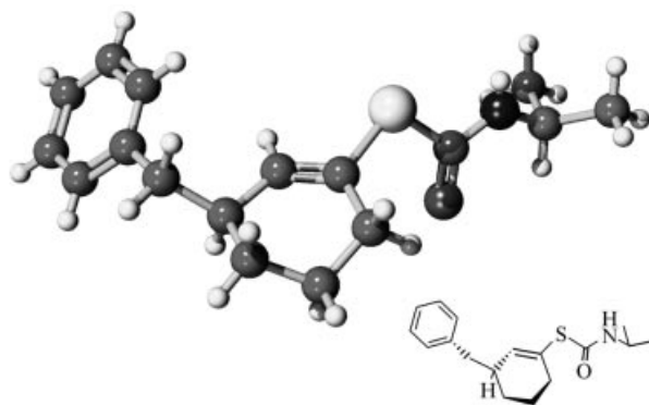
Figure 3. X-ray crystal structure of thiocarbamate (+)-( S )- 21d
