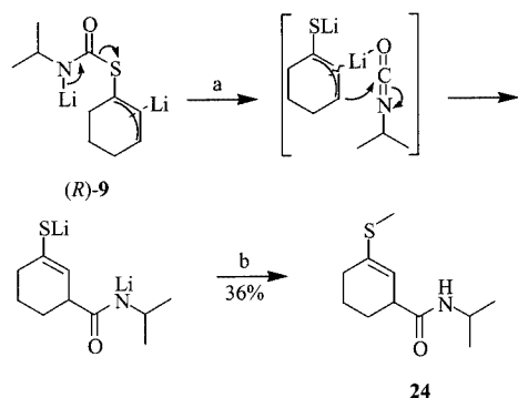
Scheme 6. Rearrangement of ( R )- 9 on warming; ligands at the lithium centers are omitted for the sake of clarity; reagents and conditions: (a) i) 10 min -78^{\circ}\text{C} ; ii) 15 min 0^{\circ}\text{C} ; iii) 15 min -78^{\circ}\text{C} ; (b) i) MeI, -78^{\circ}\text{C} , 15 h; ii) HOAc, -78^{\circ}\text{C} , 15 min; iii) \text{NaHCO}_3 (aq), 0^{\circ}\text{C}
