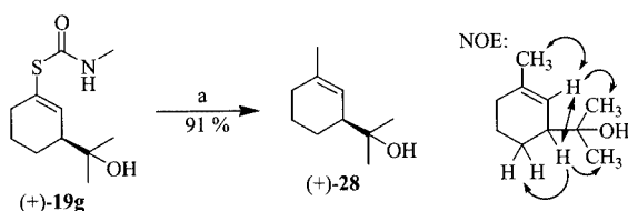
Scheme 9. Ni 0 -catalyzed cross-coupling; reagents and conditions: (a) i) 15 mol % Ni(dppe)Cl 2 , MeMgBr, toluene, 90 °C, 18 h; ii) HCl (aq)
