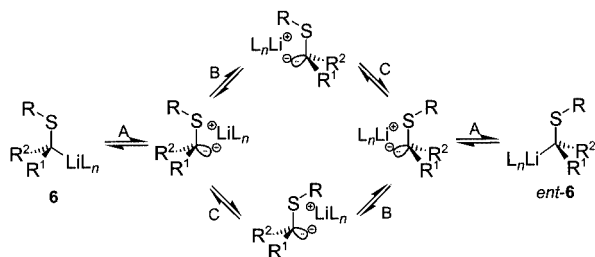
Scheme 2. Mechanism of enantiomerization
