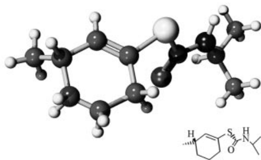
Figure 2. X-ray crystal structures of thiocarbamates ( - )-( S )- 20b and ( - )-( S )- 21b [20]
