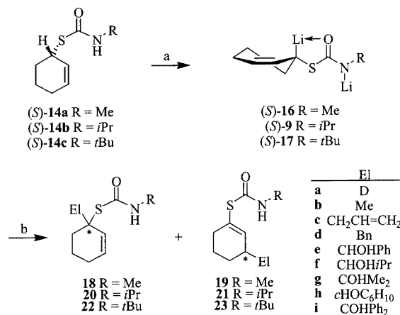
Scheme 5. Lithiation and subsequent electrophilic substitution [the ( S ) configuration for starting materials having been chosen arbitrarily]; ligands at the lithium centers are omitted for the sake of clarity; reagents and conditions: (a) s BuLi/TMEDA, –78 °C, 5–240 min; (b) i) EtX, –78 °C, 15 min to 18 h; ii) HOAc (DOAc for deuteration), –78 °C, 15 min; iii) NaHCO 3 (aq), 0 °C
