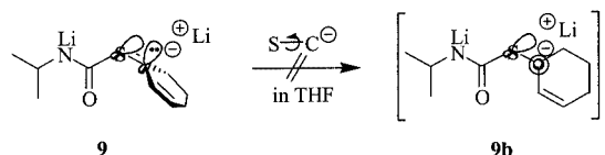
Scheme 7. Rate-determining step of racemization of dianion 9 ; ligands at the lithium centers are omitted for the sake of clarity
